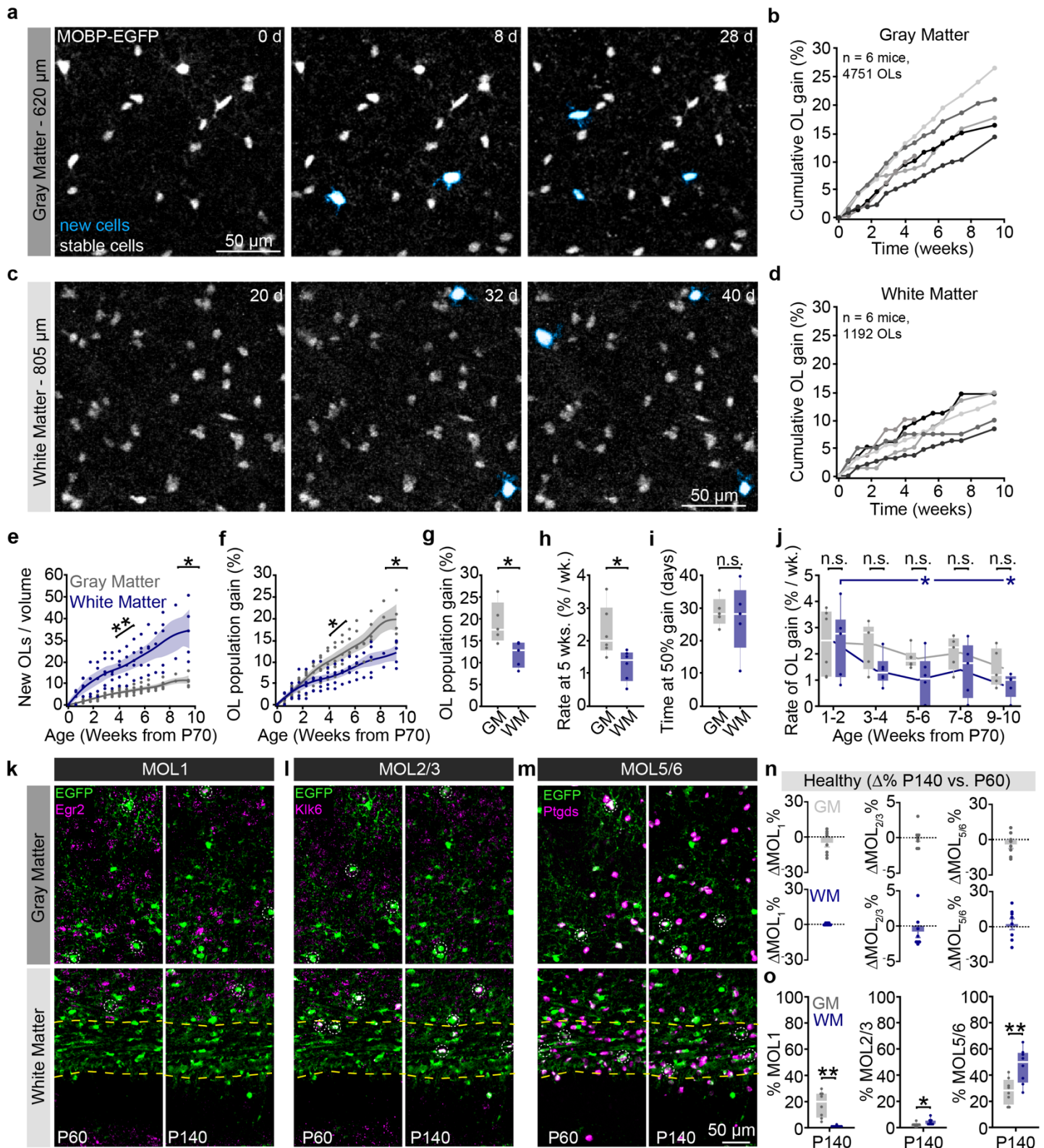
Figure 4 | Gray versus white matter differences in population growth correlate with transcriptional heterogeneity. a ) Oligodendrogenesis (cyan) over 4 weeks of imaging in layer 5 of the posterior parietal cortex (PPC). b ) Cumulative OL gain curves for individual mice over 10 weeks in the entire depth of the gray matter (GM). c ) Oligodendrogenesis in the dorsal corpus callosum over ~6 weeks of imaging in the white matter (WM). d ) Cumulative OL gain curves for individual mice in the WM. Legend Continued on next page.
