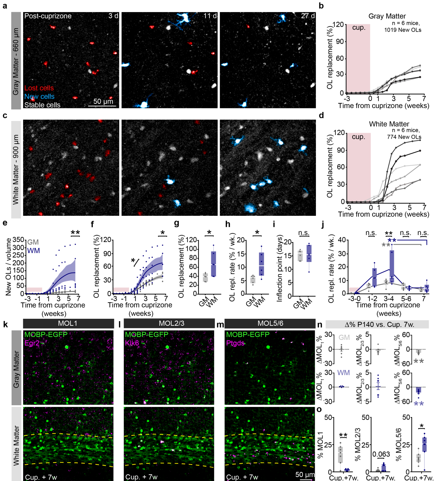
Figure 6 | Replacement of lost oligodendrocytes following cuprizone is enhanced in the corpus callosum and regional heterogeneity is partially restored through regeneration. a ) Timelapse of 24-day period after cuprizone cessation showing oligodendrocyte (OL) cell body compaction and loss (red), followed by the generation of mature myelinating OLs (cyan) in the deep posterior parietal cortex. b ) Cumulative OL replacement (% gain normalized to % loss) across the cortex for individual mice. c ) Same time points and mouse as in (a) in the corpus callosum. Figure legend continued on next page.
