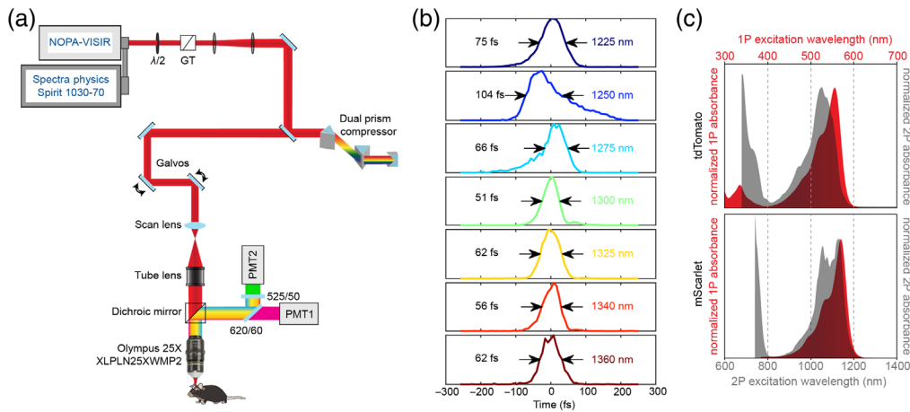
Fig. 1 Custom 3P microscope for dual-color in vivo imaging. (a) 3P light path and detection scheme for dual-color imaging. (b) Laser pulse temporal profile for wavelengths from 1200 to 1400 nm, using FROG. Pulses were characterized by the objective focus. Pulse widths indicated are the full width at half maximum (FWHM). (c) 1P and 2P excitation curves for tdTomato and mScarlet, recreated from FPbase. Note the small tdTomato excitation peak in the UV and the short wavelength 2P excitation peaks in the range of 750 to 800 nm.
